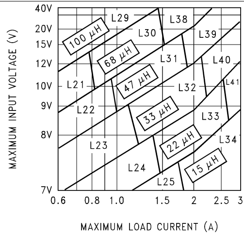
Figure 28. LM2596-5.0
