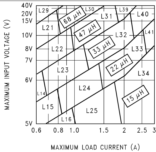
Figure 27. LM2596-3.3
