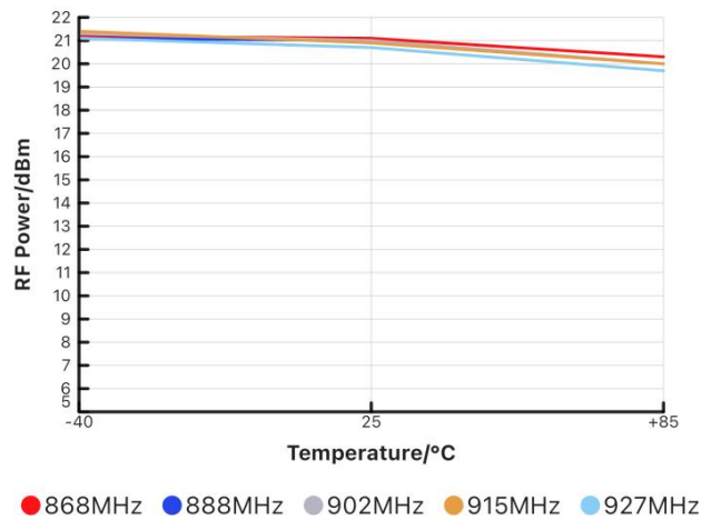
Figure 4 Max RF Power VS Temperature ( 868~927MHz )
