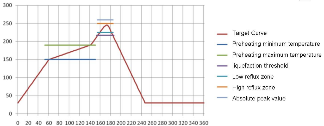
Figure 12 Reflow profile
