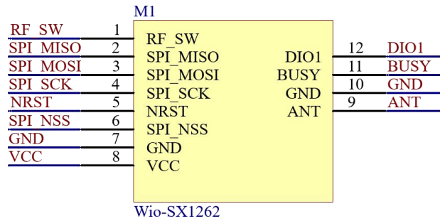
Figure 2 Wio-SX1262 Pinout
