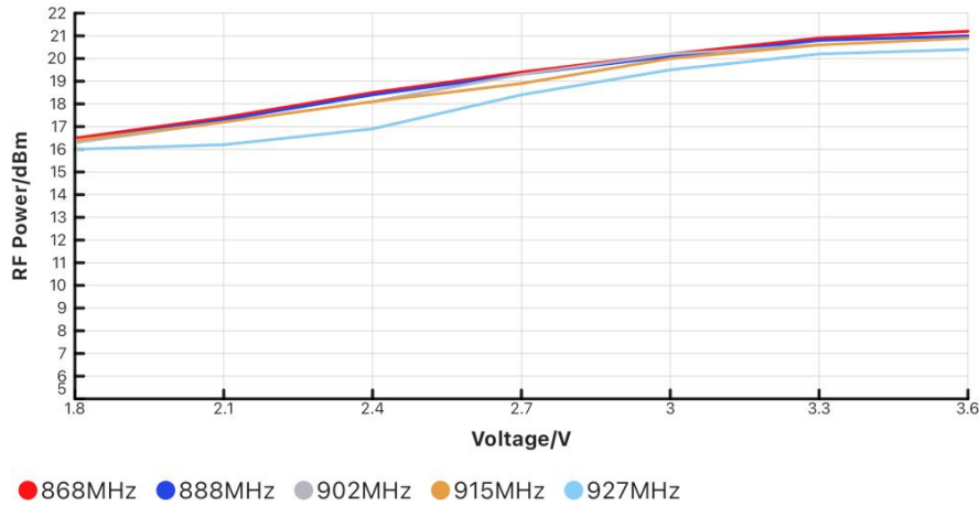
Figure 3 Max RF Power vs Voltage ( 868~927MHz )
