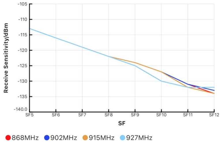
Figure 5 RF Receiver Sensitivity vs Spreading factor ( 868~927MH@BW125KHzz )
